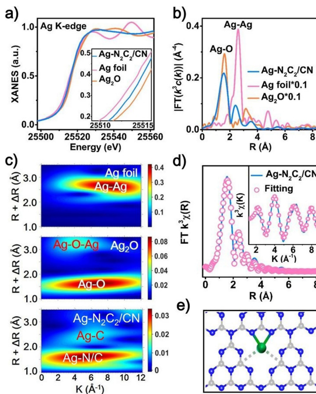
Figure 2. a) Ag K-edge XANES, b) Fourier transform of Ag K-edge EXAFS spectra, c) WT of Ag foil, Ag 2 O, and Ag-N 2 C 2 /CN. d) EXAFS fitting curve in R space and e) structure model of Ag-N 2 C 2 /CN (Ag green, N blue, C grey).
