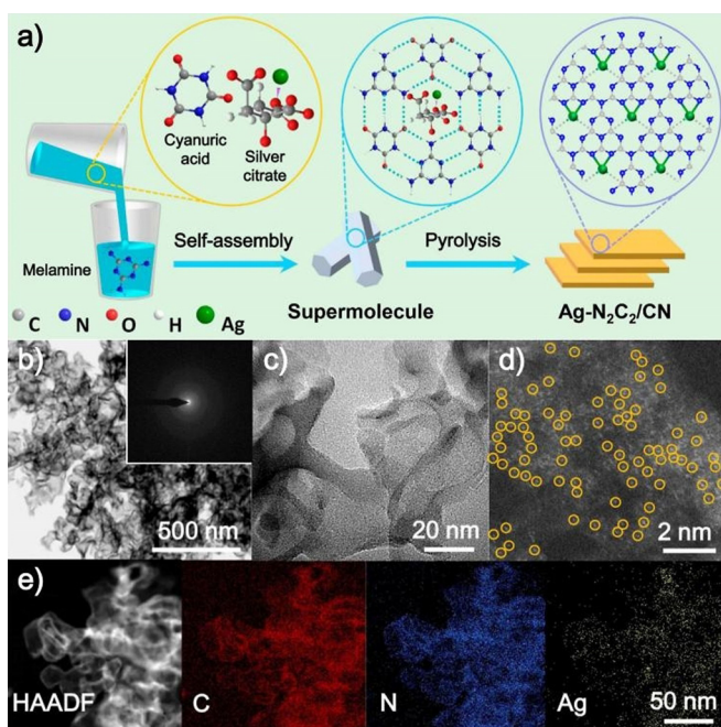
Figure 1. a) Schematic illustration of preparation of Ag-N 2 C 2 /CN, b) TEM (inset SAED), c) HR-TEM, d) AC-HAADF-STEM (the bright dots in the yellow circles are Ag single atoms), and e) HAADF-STEM with elemental mapping images of Ag-N 2 C 2 /CN.
